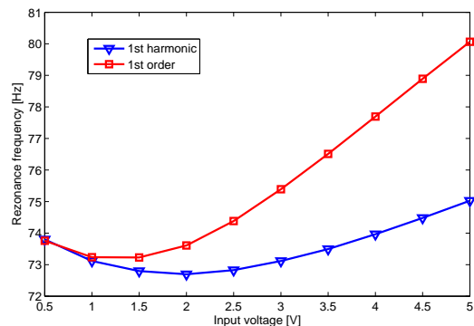
Figure 4: Estimation of resonance frequency of loudspeaker in nonlinear mode using measured data from first harmonic (blue-triangled) and from first order of Hammerstein model (red-squared) for several values of input voltage between 0.5 and 5 Volts.
